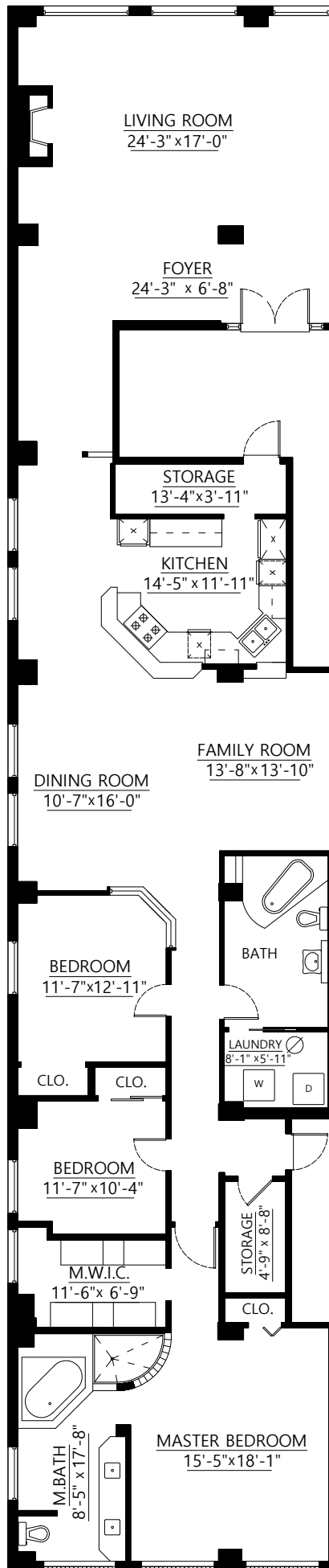
Main Floor Plan Floor Area: 2,814 sq.ft.
