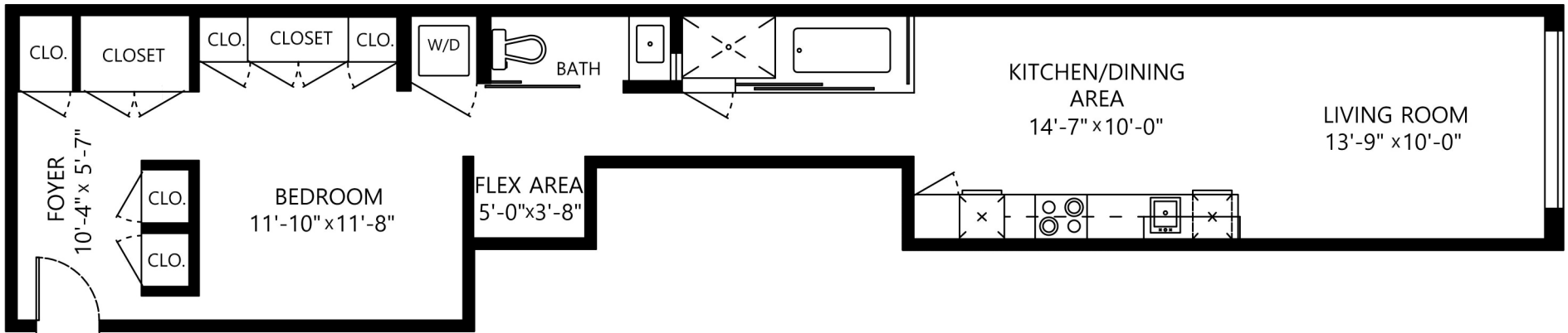
MAIN FLOOR PLAN Floor Area: 797 sq.ft. Ceiling Height: 9'-7"
